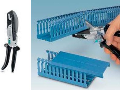
CUTFOX-CD
